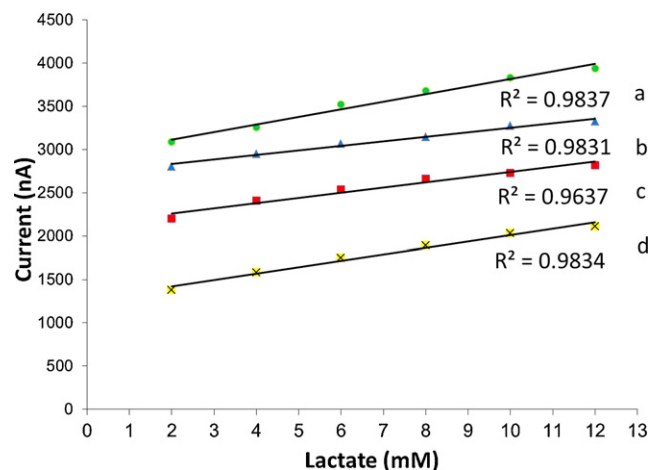
Fig. 4. Calibration curves of carbon paste-containing lactate oxidase in 0.1 M phosphate buffer (pH 5.0, 6.0, 7.0 and 7.5 are indicated by a, b, c, and d, respectively) against an outside Ag/AgCl and Pt reference and counter electrode with a detection potential of -0.15 V.
